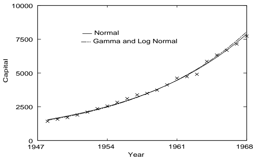
FIGURE 4.1. Fitted curves for the capital formation data in Table 4.1.
