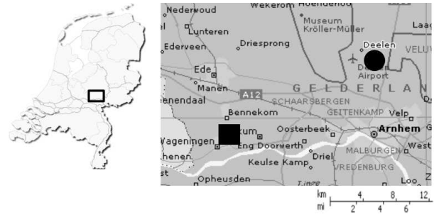
Figure 1. Indication of forecast (●) and measurement (■) location within the Netherlands
