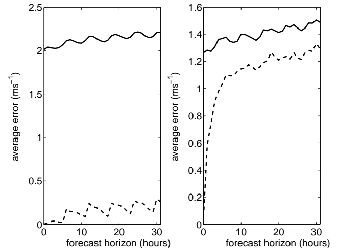
Figure 3. Average forecast error and the standard deviation of forecast error of the original forecasts (—) and of the adjusted forecasts with DBC+LAF (---) of the wind speed
