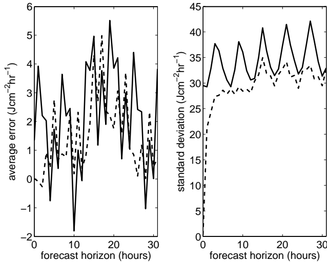
Figure 4. Average forecast error and the standard deviation of forecast error of the original forecasts (—) and of the adjusted forecasts with DBC+LAF (---) of the global radiation
