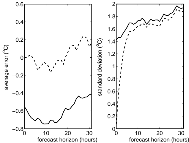
Figure 2. Average forecast error and the standard deviation of forecast error of the original forecasts (—) and of the adjusted forecasts with DBC+LAF (---) of the temperature
