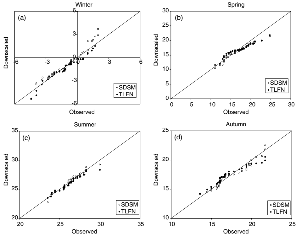
Fig. 4. Observed versus downscaled (with SDSM and TLFN) data of the 90th percentile daily maximum temperature values (°C) for each season (a-winter, b-spring, c-summer and d-autumn). Solid symbols correspond to the data downscaled with TLFN while the open symbols corresponds to the data downscaled with SDSM.
