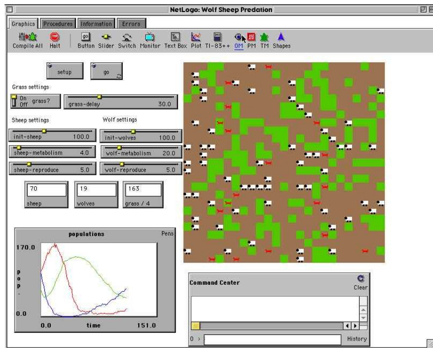
Figure 6: The NetLogo layout for the wolf-sheep predation model. In the upper left is the interface area that allows users to set model parameters and run simulations. To its right is the NetLogo graphics window that displays each individual wolf and sheep. Below the interface is a population plot window. To its right is a command center for interactively running commands.
