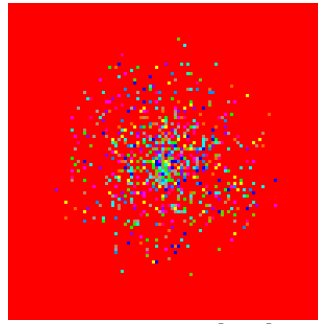
Figure 4: setpatchcolor red
