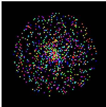
Figure 3: forward random 20
