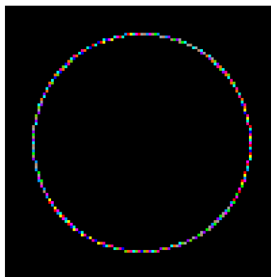
Figure 2: Forward 20
