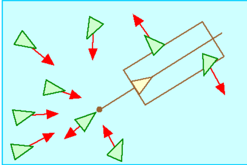
Figure 17: leader following
