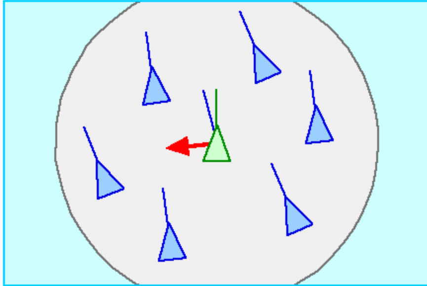
Figure 16: alignment
