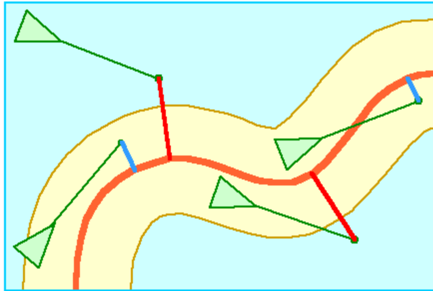
Figure 9: path following
