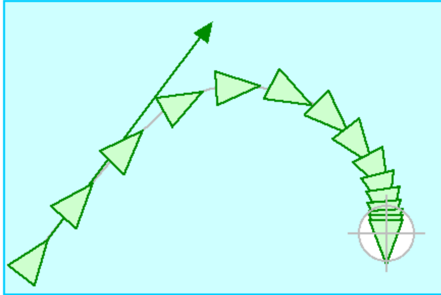
Figure 6: arrival
