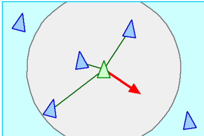
Figure 14: separation
