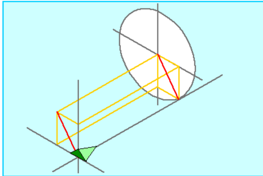
Figure 5: offset pursuit
