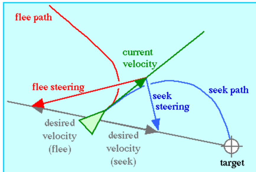
Figure 3: seek and flee
