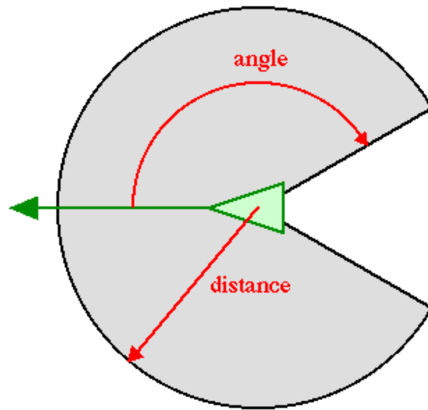
Figure 13: neighborhood
