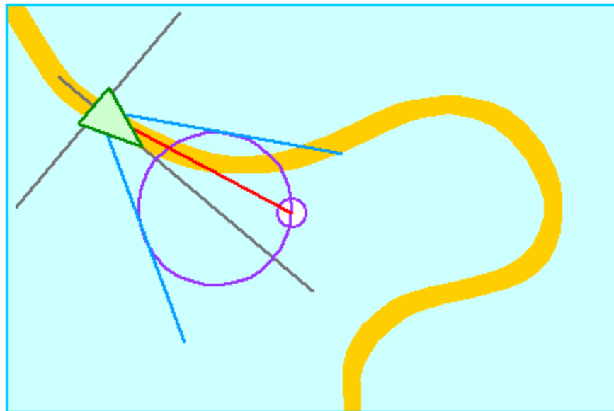
Figure 8: wander
