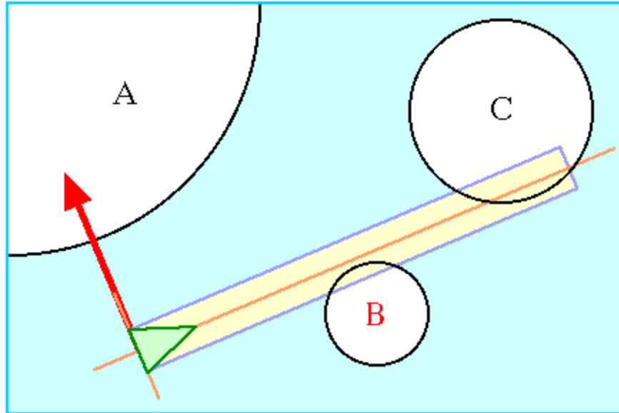
Figure 7: obstacle avoidance
