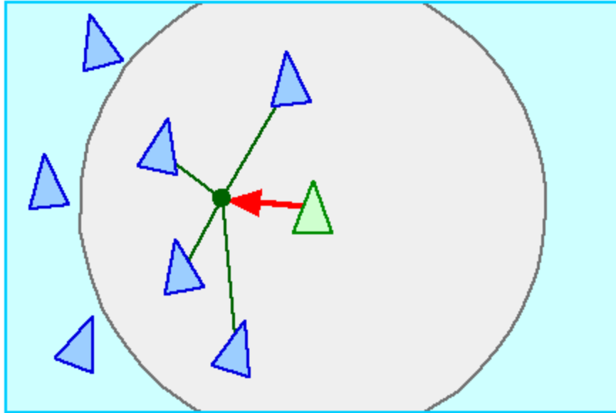
Figure 15: cohesion
