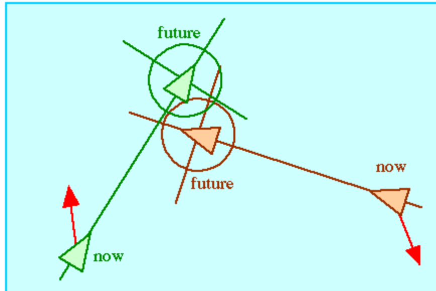
Figure 12: unaligned collision avoidance
